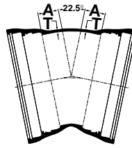
22 1/2° Bend
