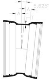
5-5/8° bend
